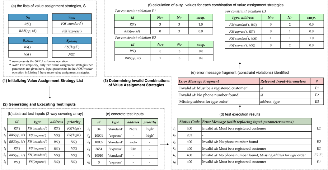
Fig. 2. The workflow of Sampling and Analyzing Error Messages in EMREST.
