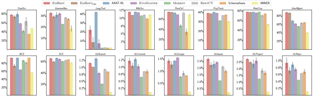
Fig. 4. Line Coverage Achieved By Different Testing Approaches
