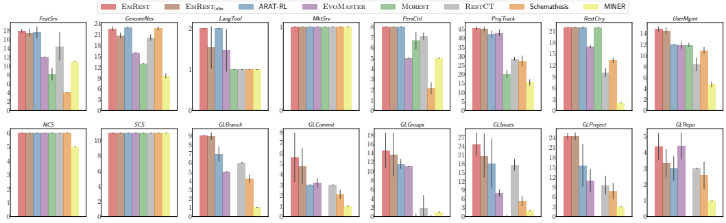
Fig. 3. Number of Operations Covered By Different Testing Approaches
