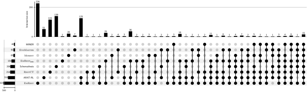
Fig. 6. Overlap of All Detected Unique Bugs Across 30 Runs
