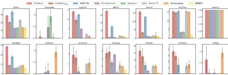
Fig. 5. Number of Unique Bugs Detected by Different Approaches (no bugs were detected in NCS and SCS )
